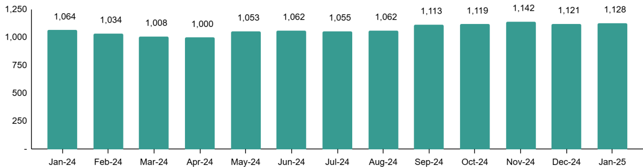
COII Vacancies
